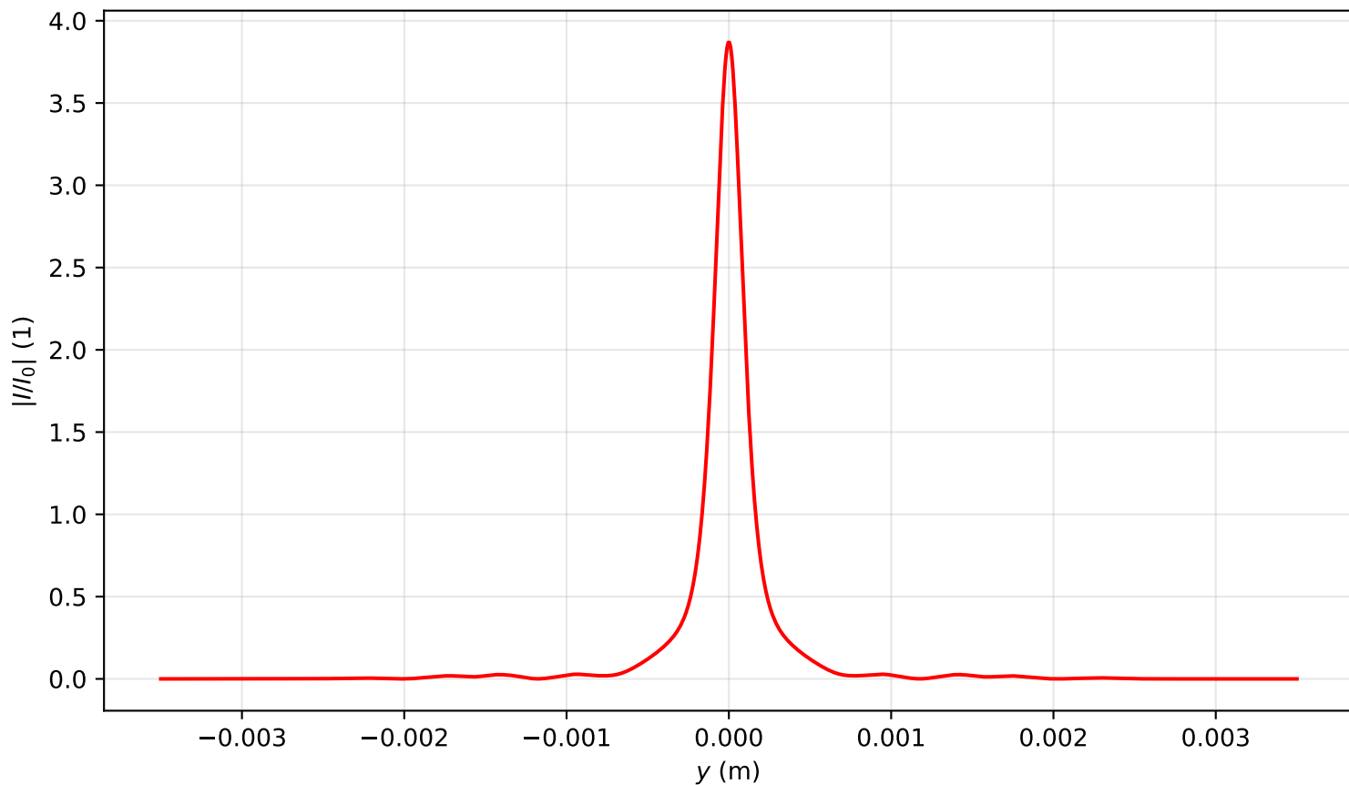
Intensity profile I(x=0, y, z=2.149)/I_0 , P_{in}=3.5P_{cr} , artificial time
